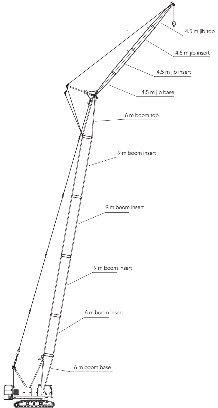
Longest boom + jib: 45 m + 18 m
